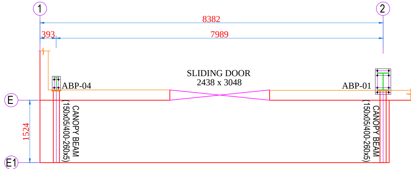
CANOPY LAYOUT PLAN
