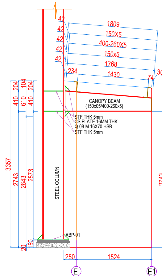
CANOPY CROSS SECTION @ 02 DETAIL (B-B)
