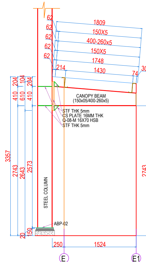
CANOPY CROSS SECTION @ 01 DETAIL (A-A)
